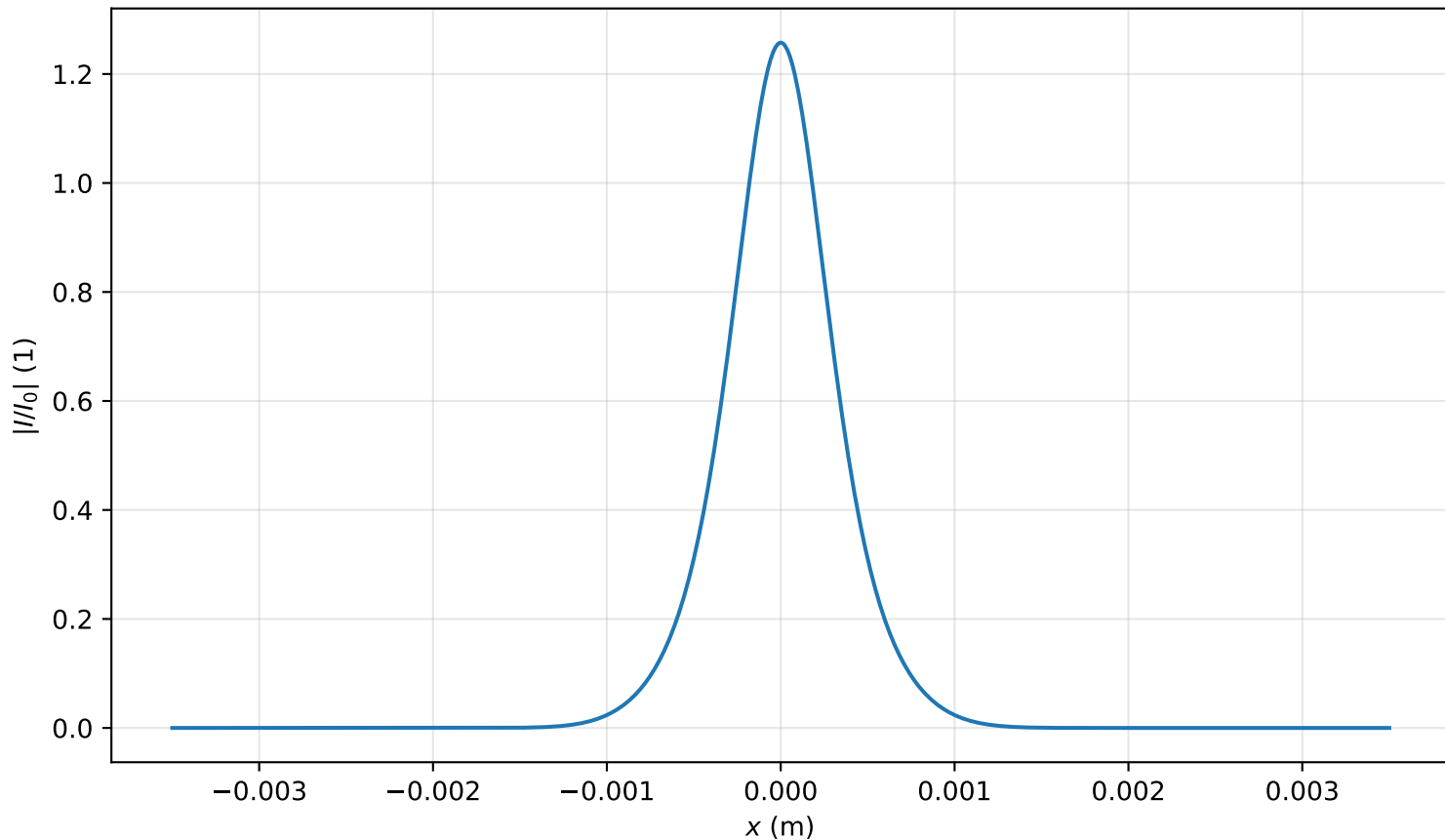
Intensity profile I(x, y = 0, z = 0.876m)/I_0 , P_{in}=0.8P_{cr} , artificial time
